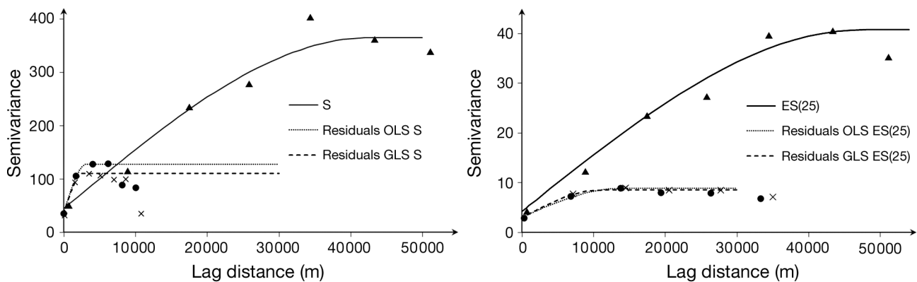
Fig. 3. Theoretical variograms of S (left) and ES(25) (right) (see Table 1) fitted to the experimental values of the diversity index and used for ordinary kriging (▲), to the residuals of the ordinary least squares (OLS) model (●), and to the residuals of the generalised least squares (GLS) model (×). The latter 2 are used for regression kriging
